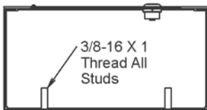
SECTION X-X
